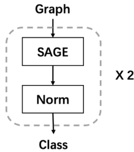
Fig. 7. Overall GraphSAGE based GNN architecture where SAGE represents the GraphSAGE module which is responsible for aggregation and Norm represents the normalization module.
